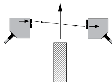
Fig. 11: Through-beam sensing
